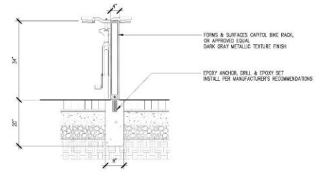
01 BIKE RACK 1" = 1'-0"
