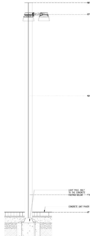
BURLINGAME CREEK PROJECTOR POLE FOOTING
