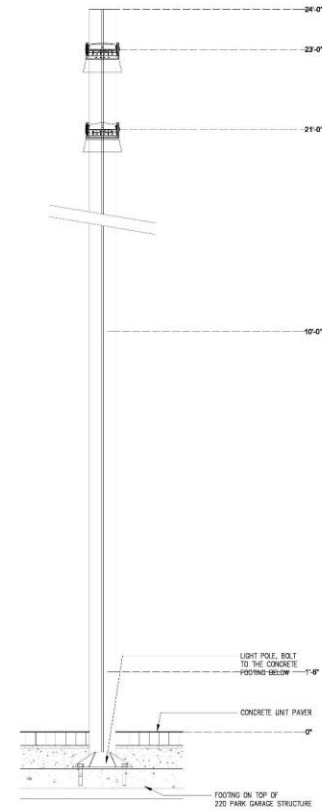
PARK ROAD "ROOM" THEATER POLE LIGHT FOOTING
