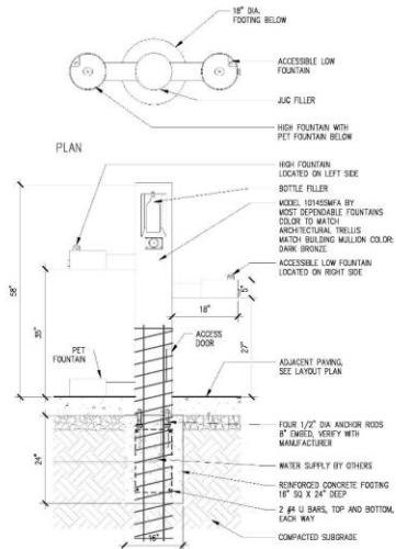
04 HYDRATION STATION 1" = 1'-0"
