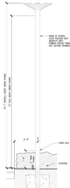
SIGNATURE POLE LIGHT FOOTING
