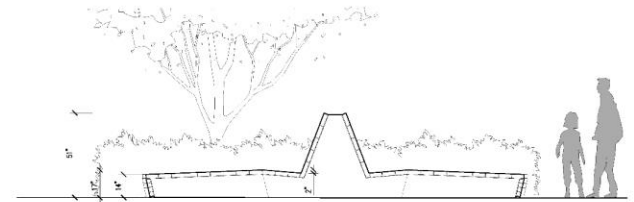
2. SECTION
