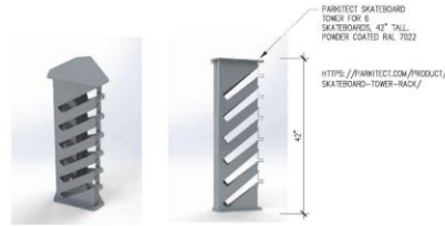
02 SKATEBOARD RACK 1" = 1'-0"
